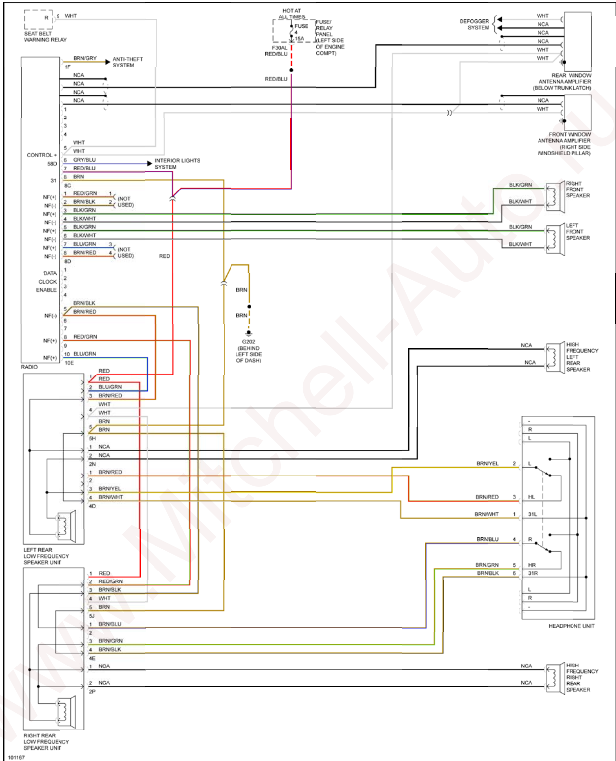
Fig. 13: Radio Circuit
